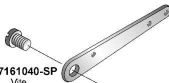
118-19315 Leva (MO-3600; MO-3900)
