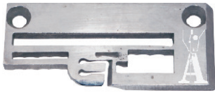
Placca 2 aghi Needle plate (2 needles) cod. 52924BH-5-8
