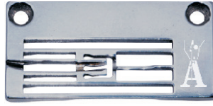
Placca 3 aghi Needle plate (3 needles) cod. E2626P (3x5,6 mm)
