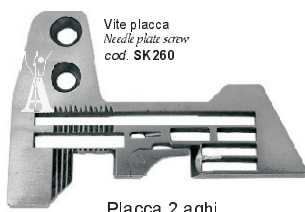
Placca 2 aghi Needle plate (2 needles) cod. E837 (3x3 mm)
