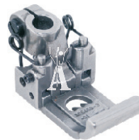
Piedino 3 aghi Presser foot (3 needles) cod. 325450-3-01 (6,0 mm)
