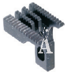
Griffa posteriore Rear feed dog cod. 321400-0-01
