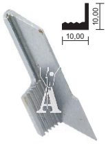
Coltello sup. dentato Upper knife for knitting cod. 209341-0-00
