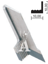
Coltello sup. widia dentato Upper knife widia for knitting cod. 209342-2-01
