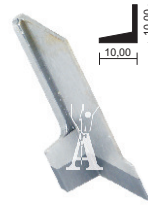
Coltello sup. widia Upper knife widia cod. 209340-2-01
