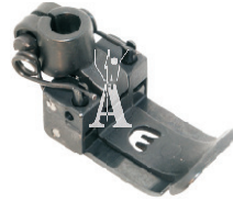
Piedino 3 aghi Presser foot (3 needles) cod. 302078-3-13 (4,5 mm) cod. 302457-3-13 (5,0 mm) cod. 300581-3-14 (6,0 mm) (= 306607-3-02)
