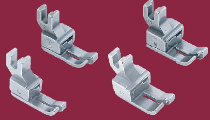
FA/N1,0 - 1,0 mm FA/N1,5 - 1,5 mm FA/N2,0 - 2,0 mm FA/N2,4 - 2,4 mm FA/N3,0 - 3,0 mm FA/N4,0 - 4,0 mm FA/N5,0 - 5,0 mm FA/N6,0 - 6,0 mm
