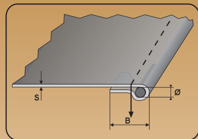
DOWNTURN LAP SEAM FOLDER WITH CORD INSERCTION
