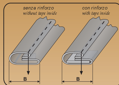
DOUBLE SHOULDER - SEW IN THE CENTRE WITH POSSIBILITY OF TAPE INSERTION
