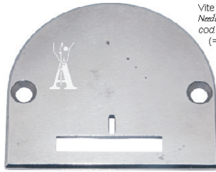
Placca - Needle plate cod. 118111-0-16
