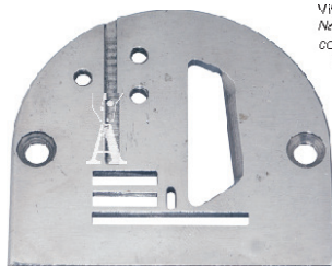
Placca - Needle plate cod. 15560
