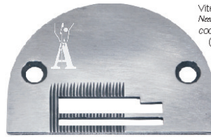
Placca - Needle plate cod. 956334-0-13
