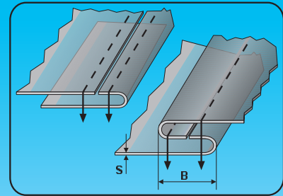
YOKE ATTACHMENT
