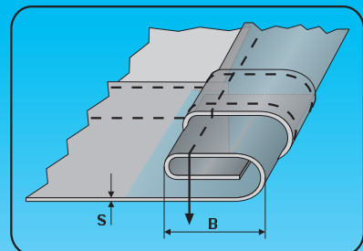
DOUBLE UPTURN SPRING HEMMER
