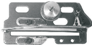
Tensione filo crochet cpl. Looper thread mechanism asm. cod. 40-3830-0
