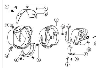
cod. 0204 000230/61 (alluminio - aluminium)
