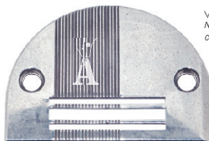
Placca rasafilo mat. fini Needle plate (thread trimmer, light mat.) cod. 0272 006501
