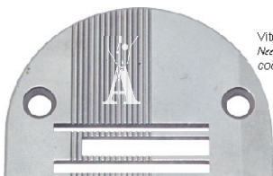
Placca rasafilo mat. medi-pesanti Needle plate (thread trimmer, medium mat.) cod. 0212 010998
