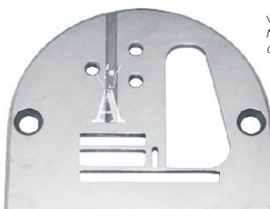
Placca rasafilo Needle plate (thread trimmer) cod. 15510
