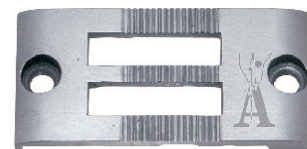
Placca due aghi - Needle plate (2 needles) cod. 0068 202710 (5,0 mm) cod. 0068 202590 (6,0 mm) cod. 0068 202600 (8,0 mm) cod. 0068 202610 (10,0 mm) cod. 0068 202670 (12,0 mm) cod. 0068 202620 (14,0 mm)
