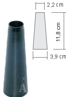
cod. 510I..8590 - rocca - bobbin winders cone
