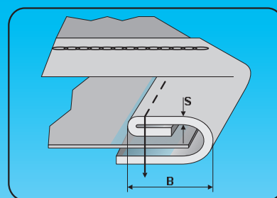
LINKING SPLIT TUBE FOLDER - THREE FOLD
